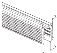
Ø 42,4 L 6000 mm U G 09.19.5042.008.00 24 8...13 09.19.5042.014.00 24 14...18 09.19.5042.022.00 24 20...22 Ø 48,3 L 6000 mm 09.19.5048.008.00 27 8...13 09.19.5048.014.00 27 14...18 09.19.5048.022.00 27 20...22
