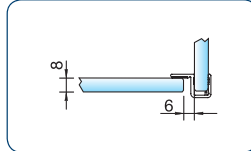
art. no. 8855KU0-8-2010 art. no. 8855KU0-8-2500 for 6 and 8 mm glass for an outward opening shower hinge
