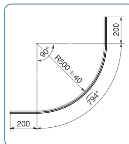
art. no. 8881E6/EV5-R500 art. no. 8882E6/EV5-R550 art. no. 8881E0/14-R500 art. no. 8882E0/14-R550
