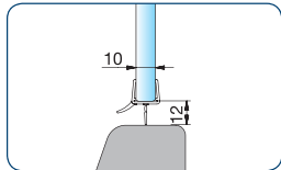
art. no. 8864KU0-12-2500 for 10 and 12 mm glass
