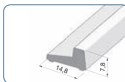
art. no. 8590E6/EV5-2010 splash protection profile square cut length 2010 mm with sealing profile 8864KU0-8-2010
