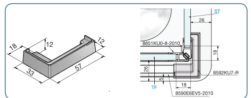
art. no. 8592KU7-R 90° cover cap right
