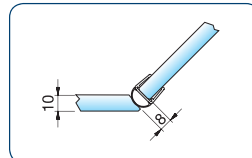
art. no. 8861KU0-12-2500 art. no. 8861KU0-12-3000 for 10 and 12 mm glass for a pendulum shower hinge
