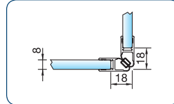
art. no. 8851KU0-8-2010 art. no. 8851KU0-8-2500 for 6 and 8 mm glass for an outward opening shower hinge
