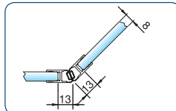
art. no. 8853KU0-8-2010 art. no. 8853KU0-8-2500 for 6 and 8 mm glass for an outward opening shower hinge
