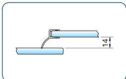
art. no. 8858KU0-8-2010 art. no. 8858KU0-8-2500 for 6 and 8 mm glass for an outward opening shower hinge
