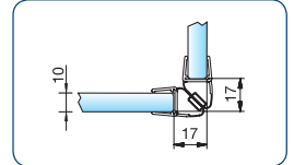
art. no. 8851KU0-12-2500 for 10 and 12 mm glass for an outward opening shower hinge
