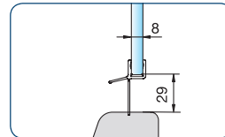
art. no. 8866KU0-8-2010 for 6 and 8 mm glass
