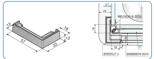
art. no. 8592KU7-L 90° cover cap left
