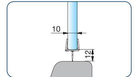
art. no. 8876KU0-12-2500 for 10 and 12 mm glass
