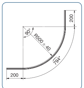
art. no. 8867KU0-8-R500 curved for tube radius R500 - 550 for 6 and 8 mm glass winding off = 1194 mm
