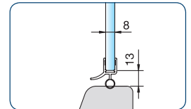
art. no. 8863KU0-8-2010 for 6 and 8 mm glass
