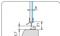
art. no. 8868KU0-8-R500 for 6 and 8 mm glass in combina- tion with curved splash guard for tuberadius R500-550 winding off = 1194 mm (art. no. 8881 and 8882-R500)
