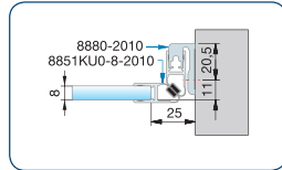
carrier profile for door stop
