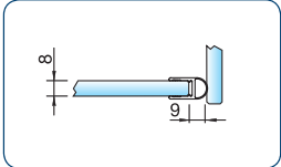
art. no. 8861KU0-8-2010 art. no. 8861KU0-8-2500 for 6 and 8 mm glass for an inward and outward opening shower hinge
