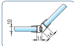
art. no. 8875KU0-12-2500 for 10 and 12 mm glass for an inward and outward opening shower hinge
