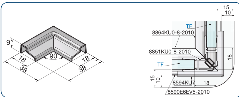
art. no. 8594KU7 90° corner connector
