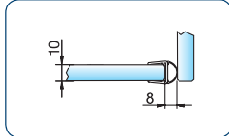
art. no. 8861KU0-12-2500 art. no. 8861KU0-12-3000 for 10 and 12 mm glass for an inward and outward opening shower hinge
