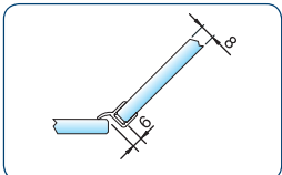
art. no. 8860KU0-8-2010 art. no. 8860KU0-8-2500 for 6 and 8 mm glass for an inward opening shower hinge
