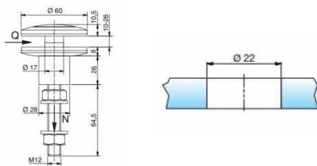
Punkthalter Edelstahl (A4) Point fixture stainless steel (316)
