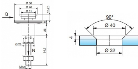
Punkthalter Edelstahl (A4) Point fixture stainless steel (316)
