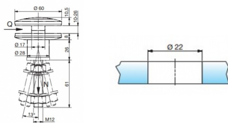
Punkthalter Edelstahl (A4) Point fixture stainless steel (316)
