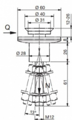
Punkthalter Edelstahl (A4) Point fixture stainless steel (316)
